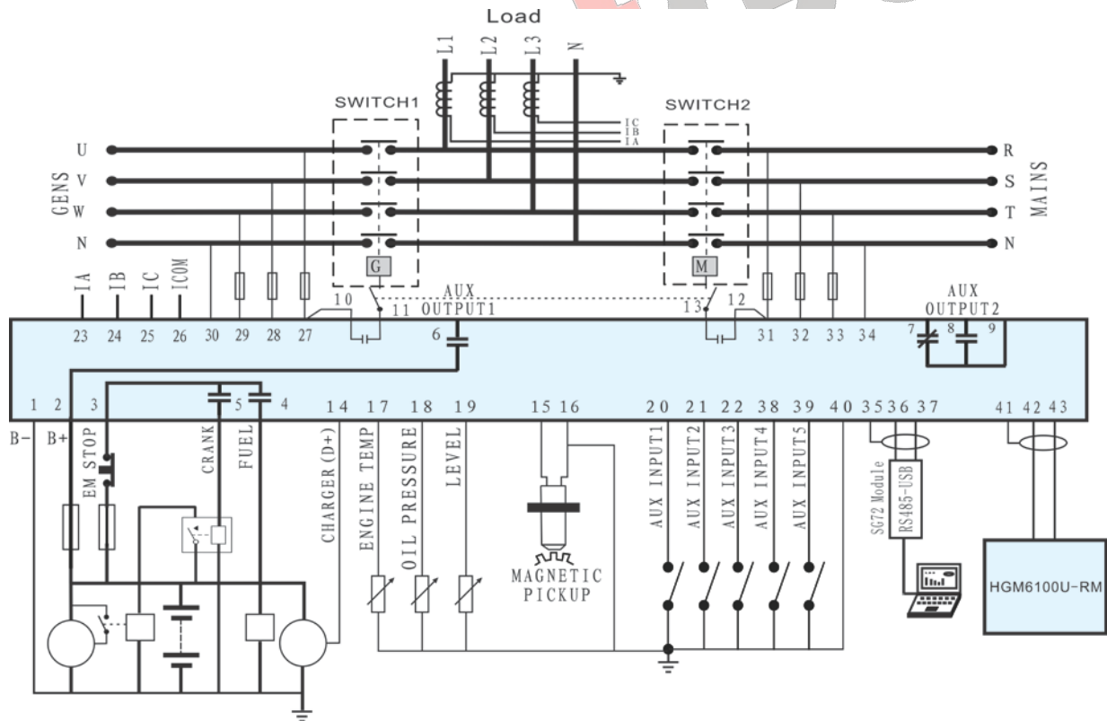
HGM6110U2C Typical Application Diagram
