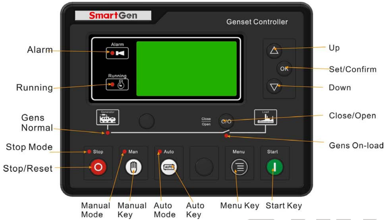
HGM6110U2C Panel Indicators
