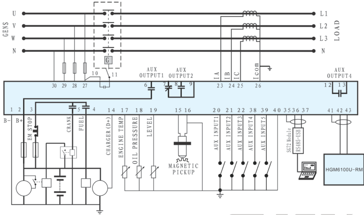
HGM6110U2C Typical Application Diagram
