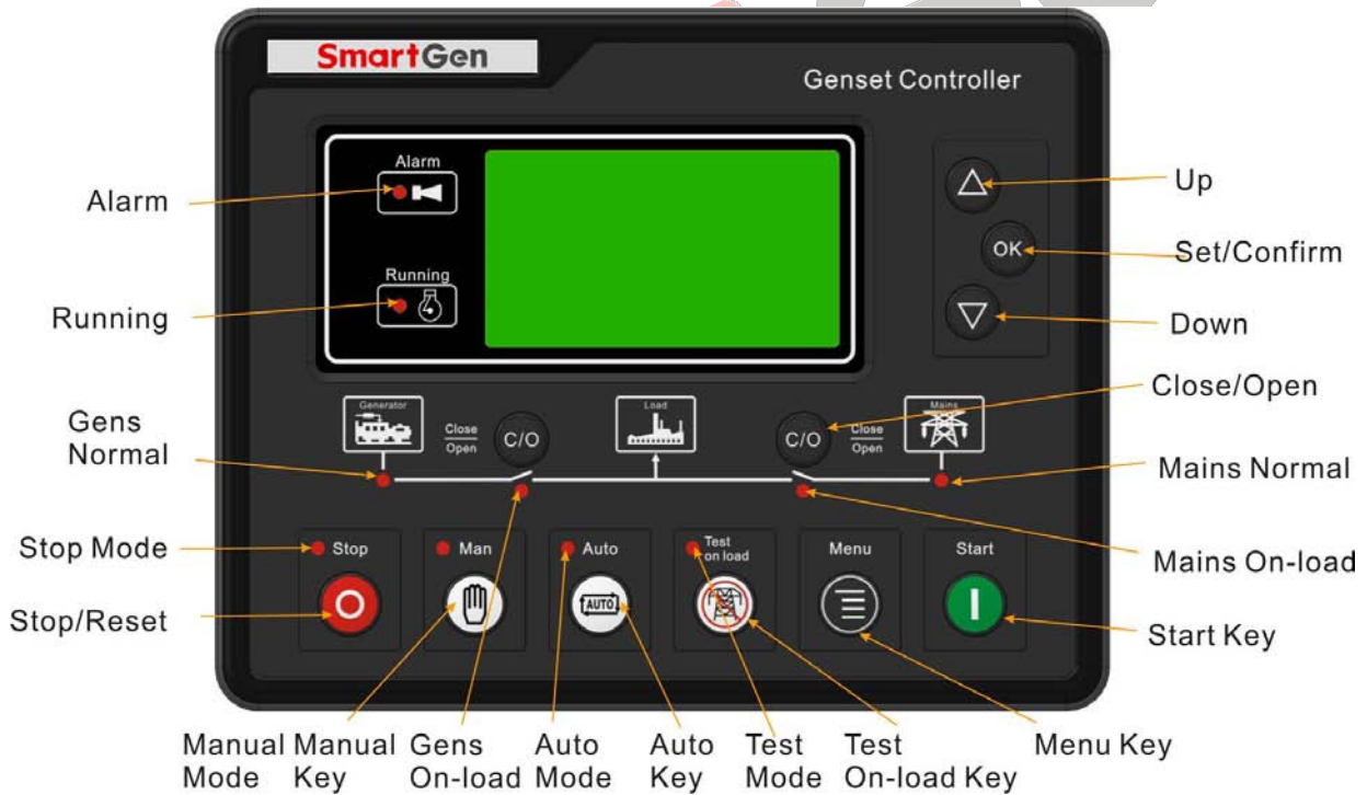
HGM6120U2C Panel Indicators
