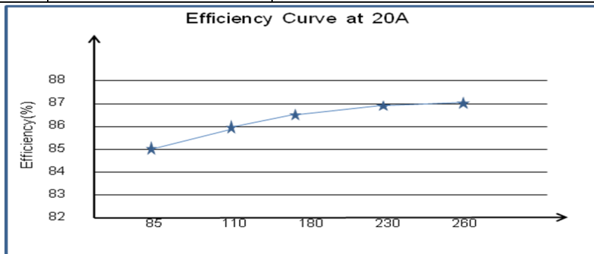
Fig. 3 Efficiency Curve
